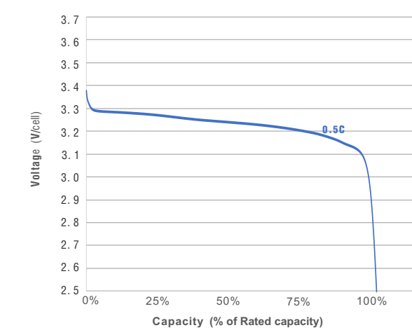
Dierent Discharge Rate and Temperature Characteristic
