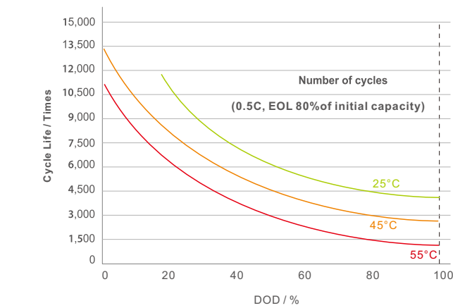
Typical Cycle Life
