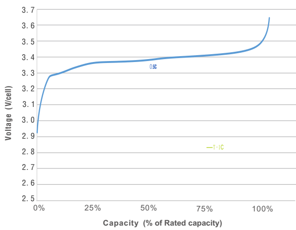
Dierent Charge Rate and Temperature Characteristic
