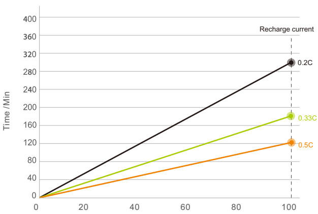
Typical Recharge Time
